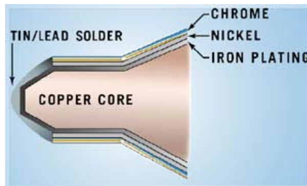
Cross-section of typical solder tip, with lead-free the solder is lead-free
